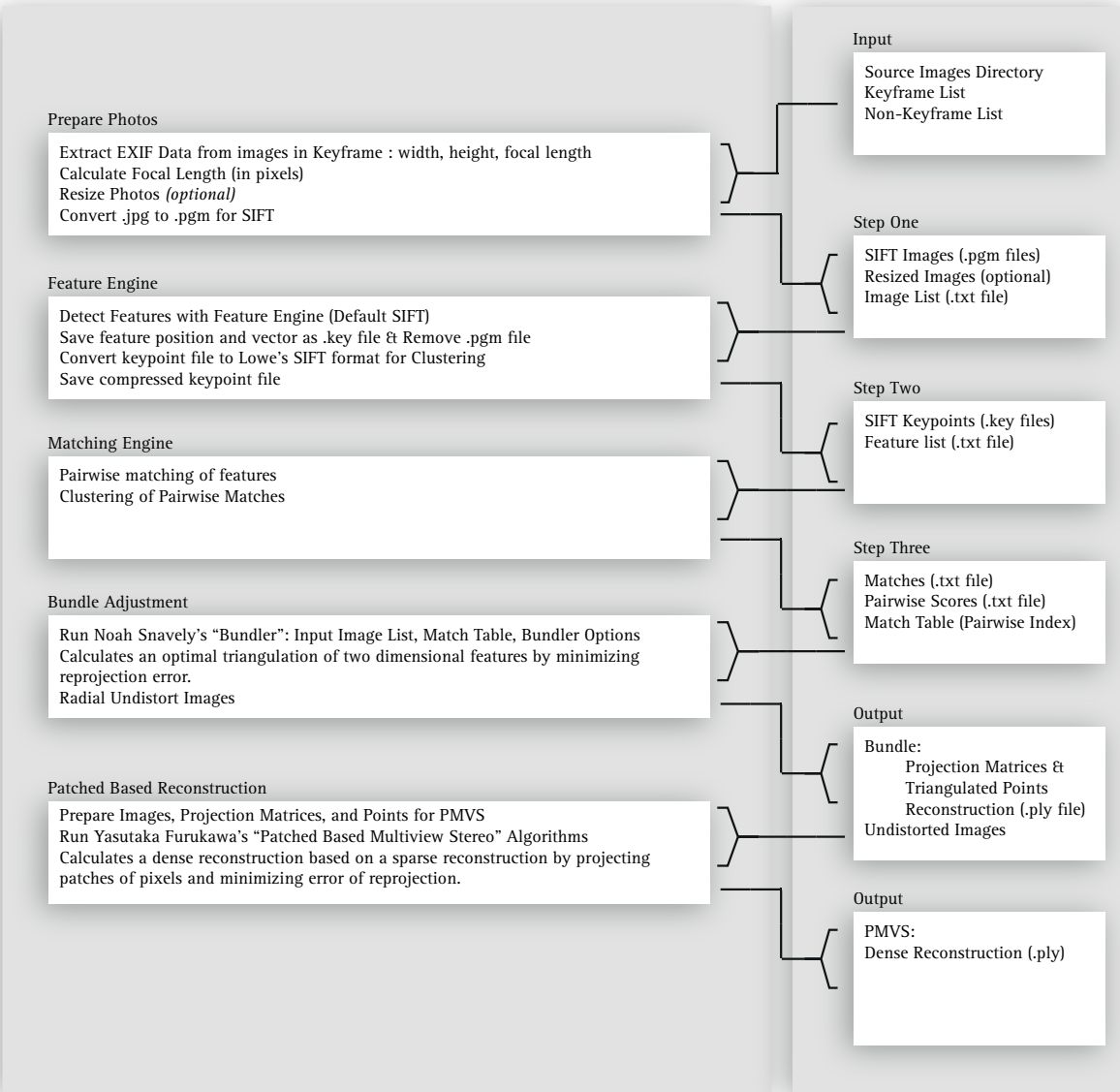
Figure 71: Diagram of the Structure from Motion Pipeline. The gray box on the left shows the program flow of the SfM Pipeline. The gray box on the right shows the input and output files of the SfM Pipeline at various stages in the process. This process begins with input from the Two Dimensional Browser.
