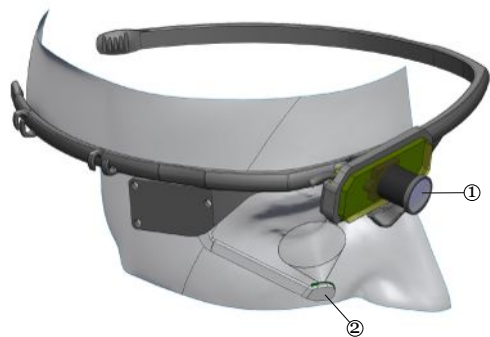
Figure 43: Second headset prototype. Pictured here with a mount accommodating a Logitech C525 Webcam [1] as the world facing camera, and a Omnivision Camera-Cube as the eye facing camera [2].
