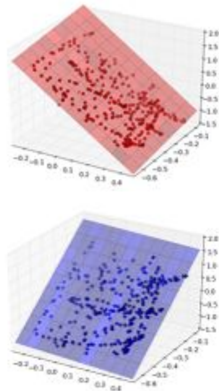
Figure 55: First order multivariate polynomials result in simple planes which poorly fit the data.
