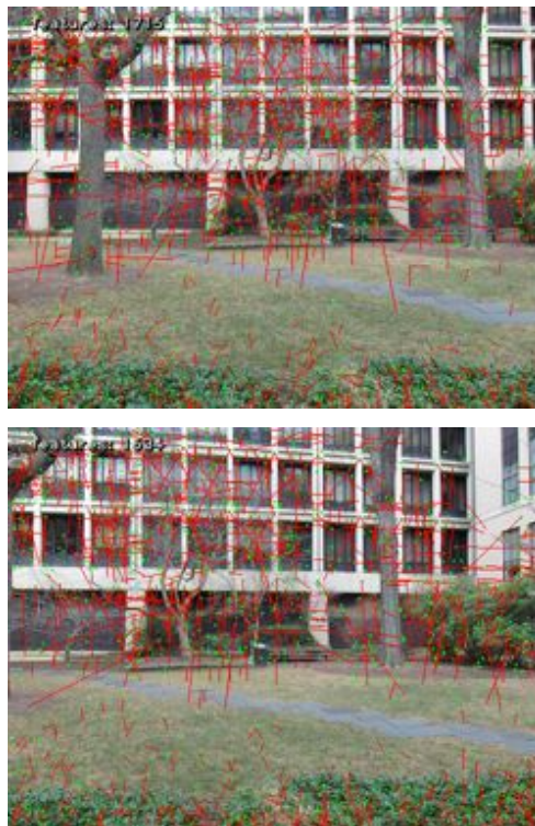
Figure 63: Two images that show SIFT key points as green dots for two views of a courtyard at MIT, images are separated by ten degrees in rotation about the Z axis. The red lines represent the scale and orientation of each key point. The number of key points found in each image is listed in the top left corner of each image. It is possible with visual inspection alone to locate some matched features.
